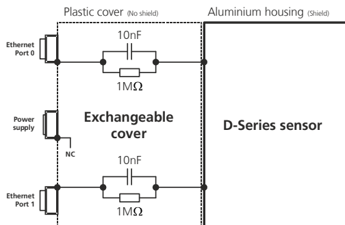
Figure 7: Shielding concept of the D-Series sensor and the exchangeable cover with Industrial Ethernet
