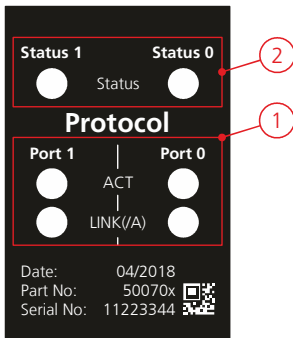
Figure 8: Status LED's on exchangeable cover with Industrial Ethernet
