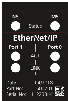
Figure 11: EtherNet/IP™ status LED's
