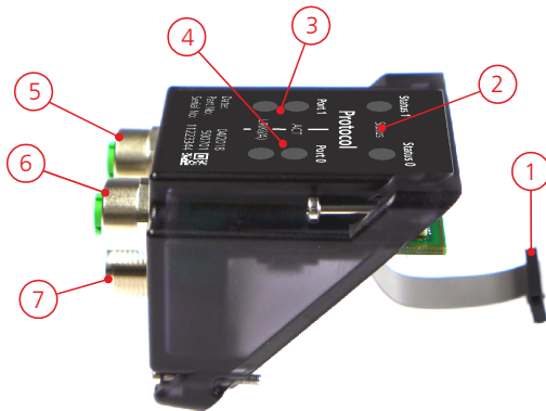
Figure 3: Overview electrical components of the exchangeable cover with Industrial Ethernet
