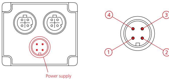
Figure 4: Connection diagram of the sensor power supply
