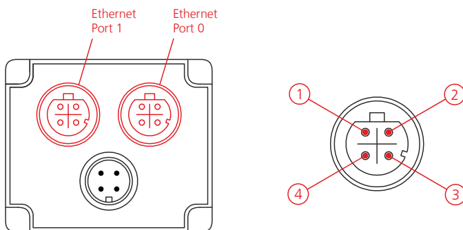
Figure 5: Connection diagram of the Ethernet port 0 & 1
