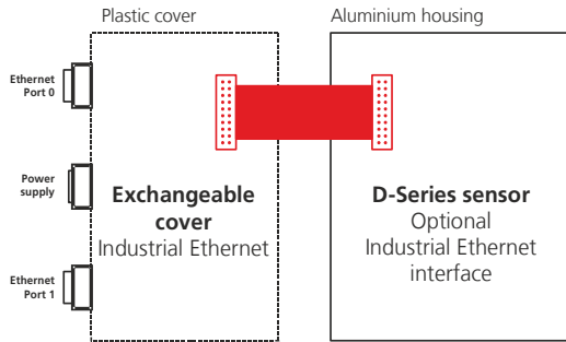
Figure 6: Connection diagram of exchangeable cover with Industrial Ethernet and D-Series sensor
