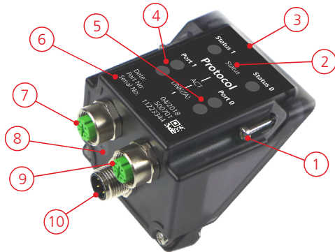
Figure 2: Components with detail information of the exchangeable cover with Industrial Ethernet
