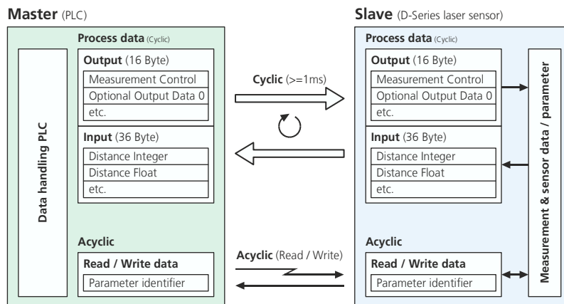
Figure 9: Cyclic (Process data) and acyclic communication between Industrial Ethernet Master (PLC) and the D-Series device with Industrial Ethernet interface.
